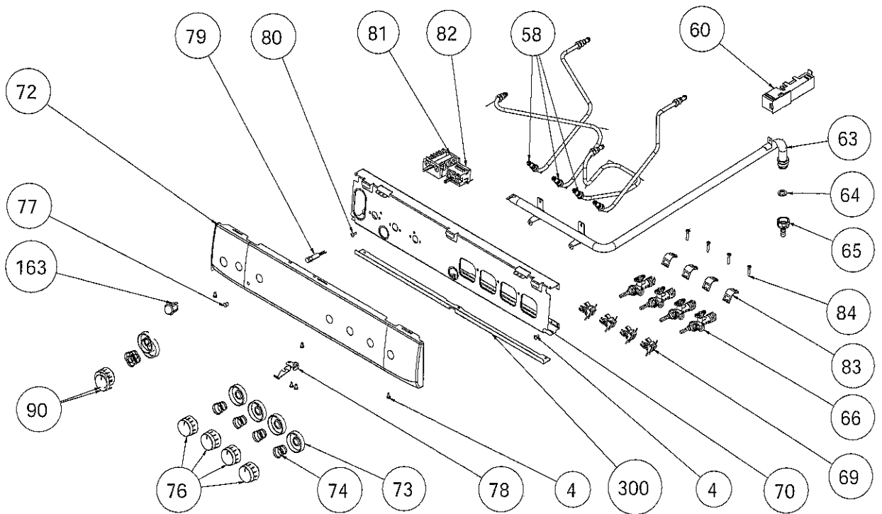
3D- 4GAS - NO TIMER CONTROL PANEL ASSEMBLY
